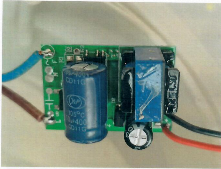
Component View
